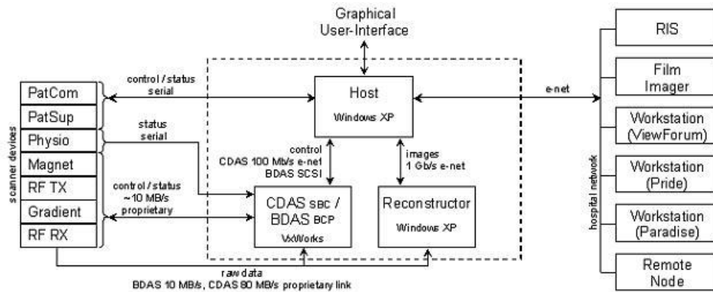
Figure A.1: Main MR system components and their physical connections
