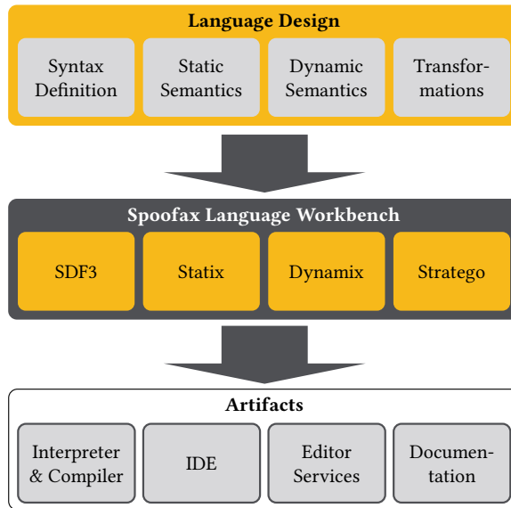
Figure 1.3: High-level idea of the Spoofax Language Designer's Workbench (Visser, Wachsmuth, et al., 2014), where aspects of the language are defined declaratively using meta-DSLs from which multiple artifacts are automatically derived.
