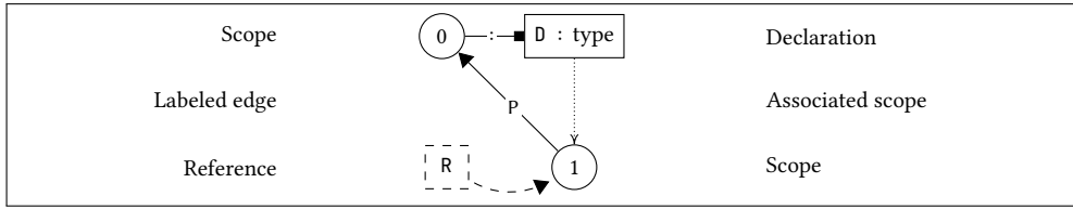
Figure 2.1: Overview of the notation used for scope graphs in this chapter.
