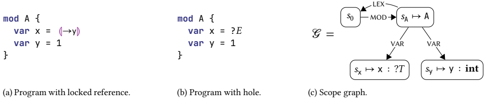
Figure 4.5: Small example program and its scope graph.
