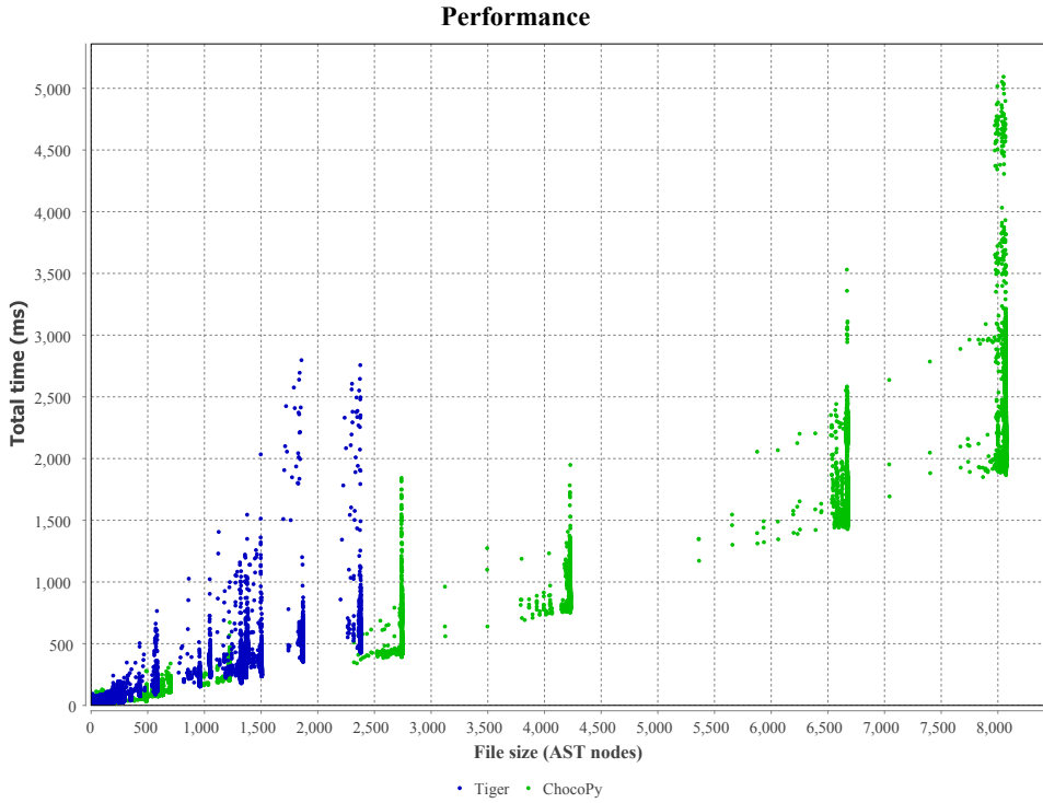
Figure 3.10: Code completion algorithm performance as a scatter plot, showing the time spent on each of the 60 624 Tiger and ChocoPy code completion invocations against the number of AST nodes in the test file.
