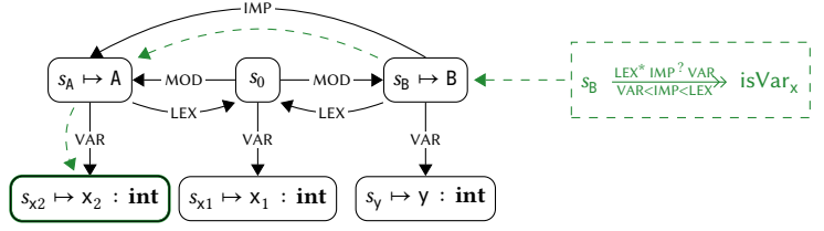
(b) Scope graph for the program in Fig. 4.3a.
