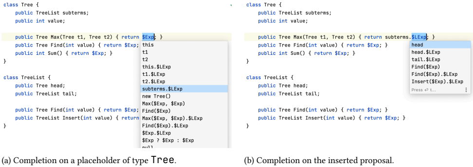
Figure 3.1: Code completion in action: the user invokes code completion on the selected placeholder and gets presented a complete list of completion proposals that are syntactically and semantically sound.
