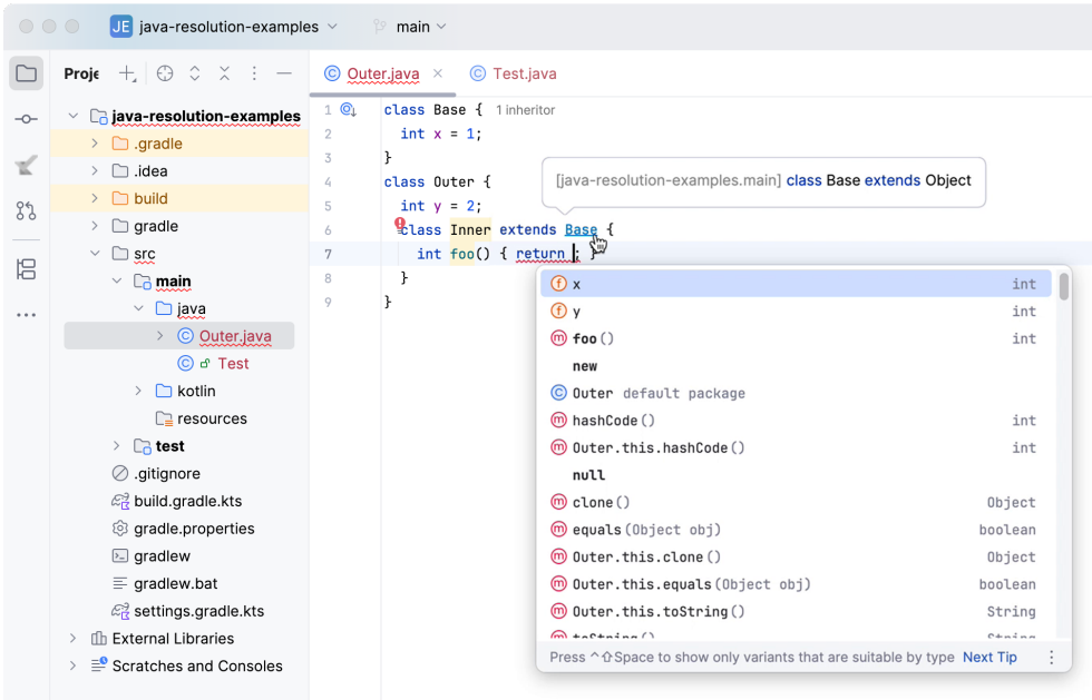
Figure 1.1: The IntelliJ IDEA development environment showing syntax highlighting, code completion, warning and error markers, hover type information, a quick-fix button, among other editor services. The user is about to navigate to the Base class definition by clicking its usage in the code.
