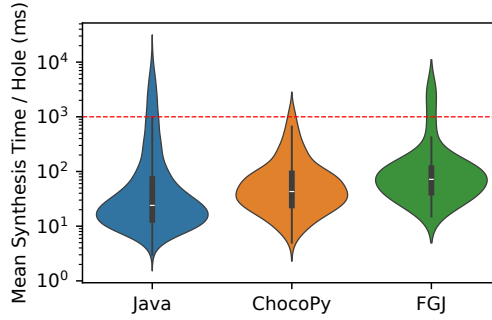
Figure 4.13: Logarithmic plot of the time spent synthesizing references per hole in each of 2575 successful test cases. The dashed red line marks 1 second.
