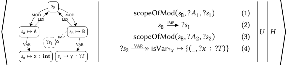
Figure 4.10: Example program (top-left) and intermediate synthesis state (below and top-right).
