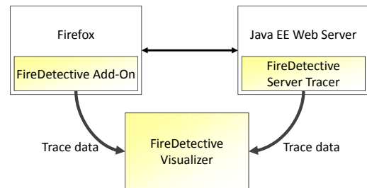
Figure 1: Architecture of FireDetective.
